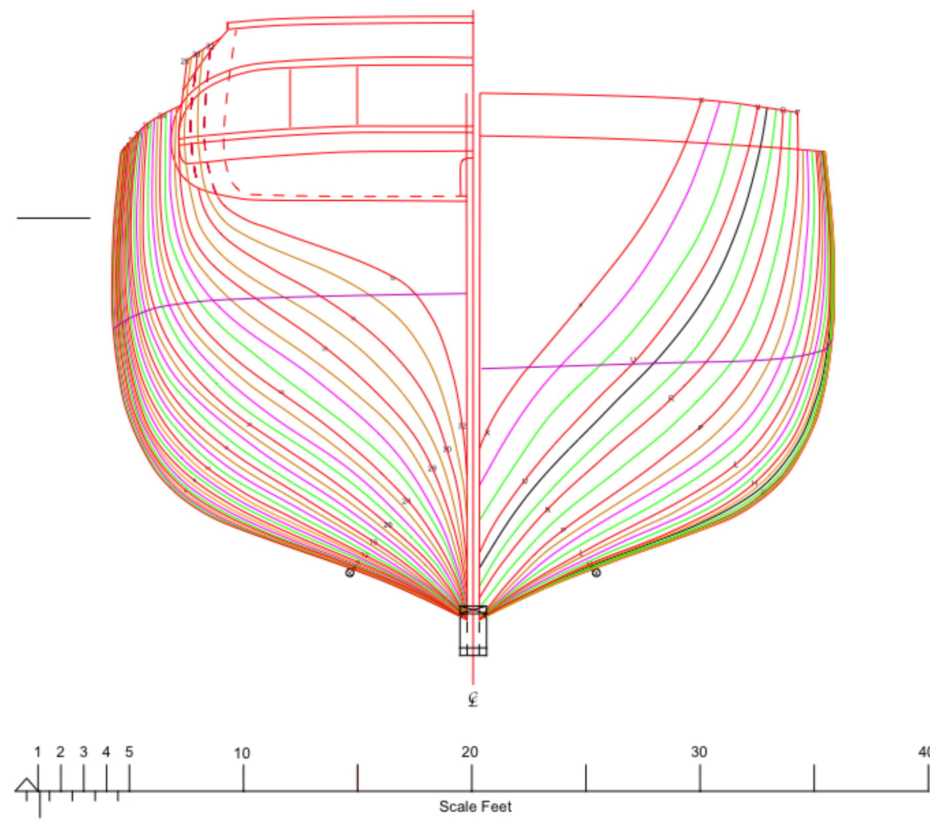
United States Sloop Peacock (1813) Body Plan
