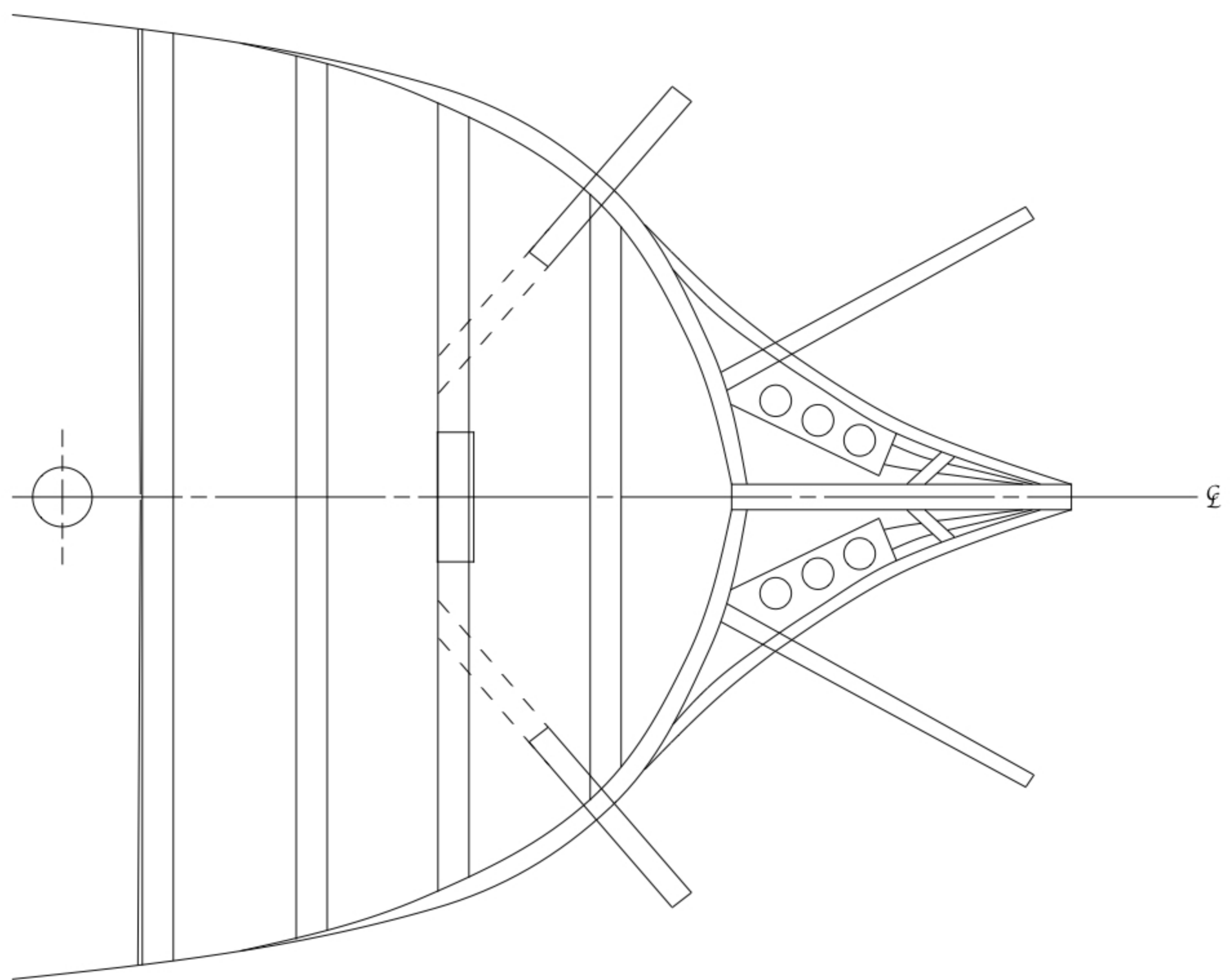
Forecastle Deck Framing
